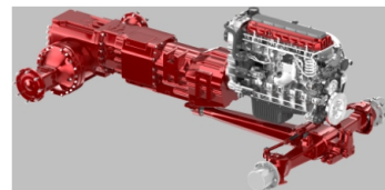
tractordetails_diesel_14
