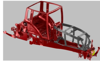
tractordetails_diesel_17
