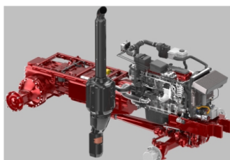
tractordetails_diesel_12
