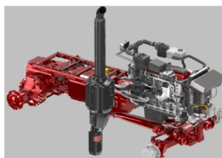
tractordetails_diesel_13
