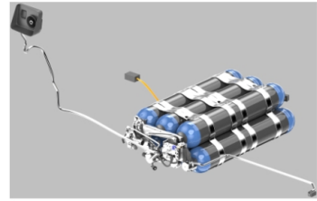
Hydrogen_Elements
