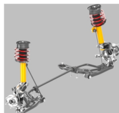
Front_Suspension
